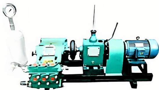
BW150注浆泵
